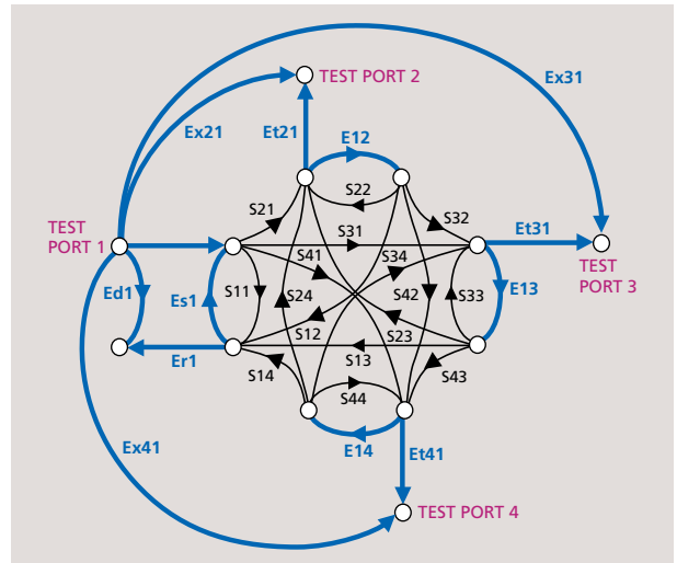
Error Model of 4-port Device
