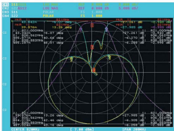
4-channel, 6-trace display with ANNOTATION ON, MENU OVERLAY OFF, SCALE UP OFF
