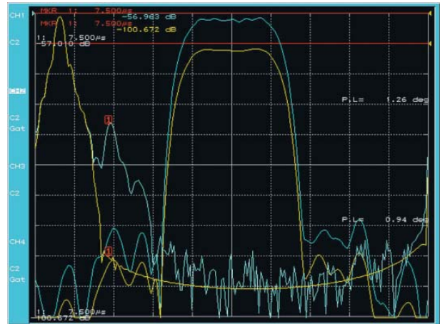
Comparison of GATE ON and GATE OFF at Frequency Axis and Time Axis
